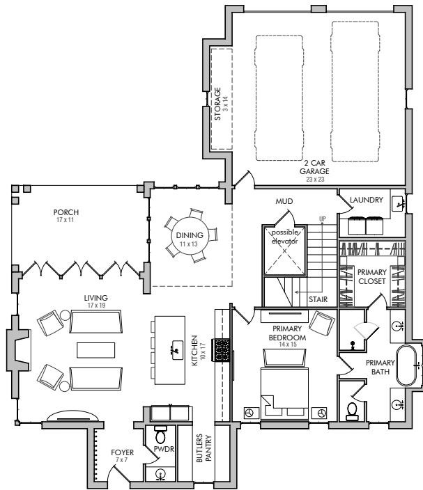
FIRST FLOOR PLAN 3/32"=1'-0"
